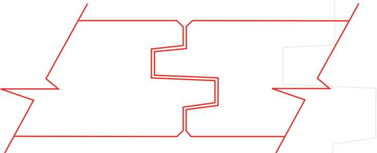
5/4 X 5 DECKING - GROOVED (JEM) ▶1.02 x 4.65 ▶ Installation - T6 hidden clip
