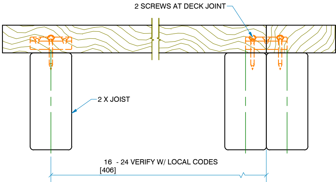
SECTION: LAYUP SIDE VIEW
