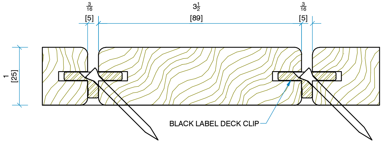
SECTION: LAYUP END VIEW
