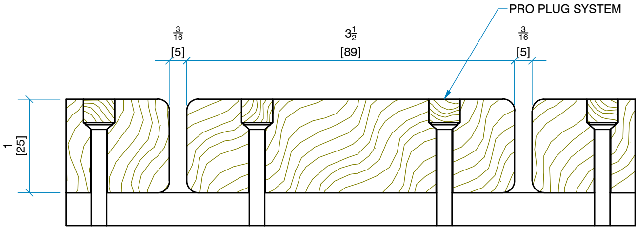
SECTION: LAYUP END VIEW
