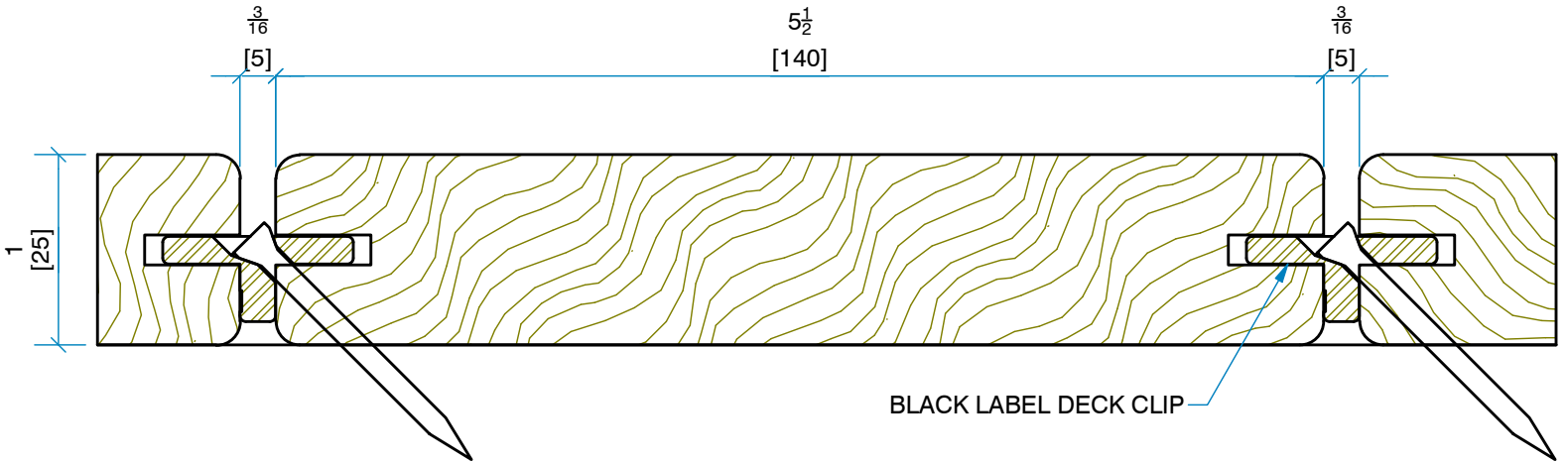
SECTION: LAYUP END VIEW
