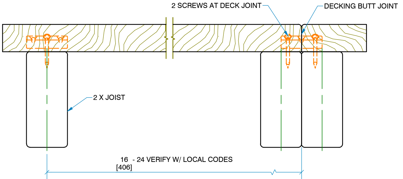
SECTION: LAYUP SIDE VIEW
