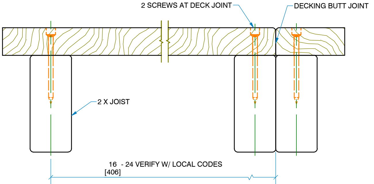
SECTION: LAYUP SIDE VIEW
