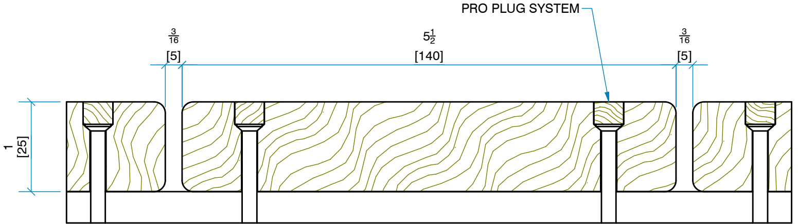
SECTION: LAYUP END VIEW
