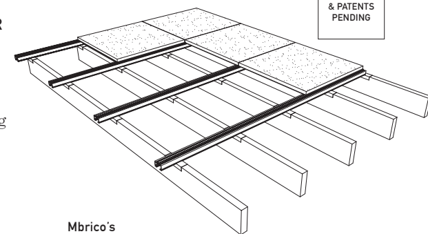
Mbrico's revolutionary track system applies to standard deck framing
