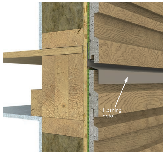
Fig.22 - Horizontal joint
