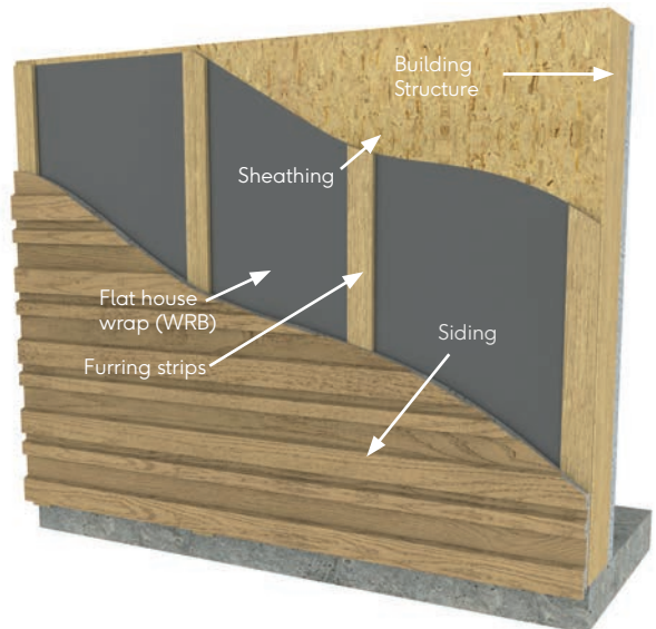
Fig.4 - Typical wall build-up with furring strips
