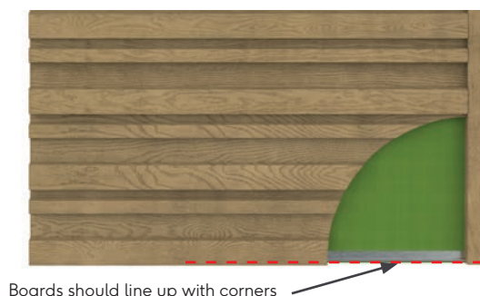
Fig.17 - Height of starter trim
