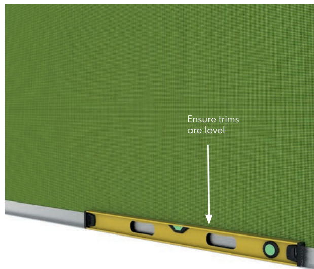
Fig.16 - Installing starter trim
