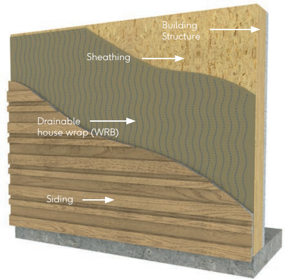
Fig. 2 - Typical wall build-up with drainable housewrap
