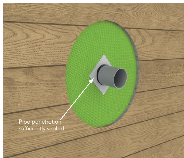
Fig.30 - Wall penetration
